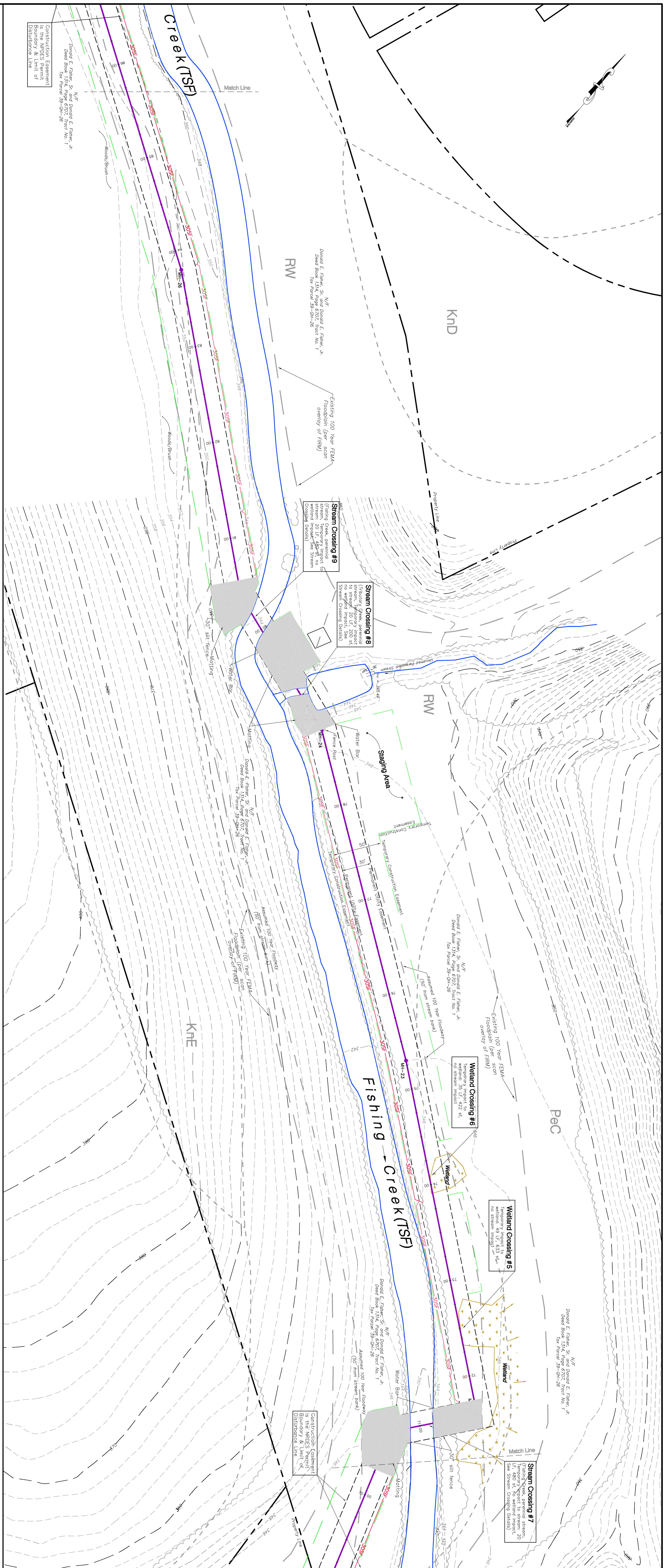
SANITARY SEWER INTERCEPTOR PLAN VIEW SCALE: 1" = 30'
