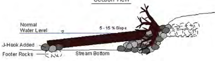
Section View
