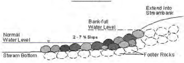
Section View
