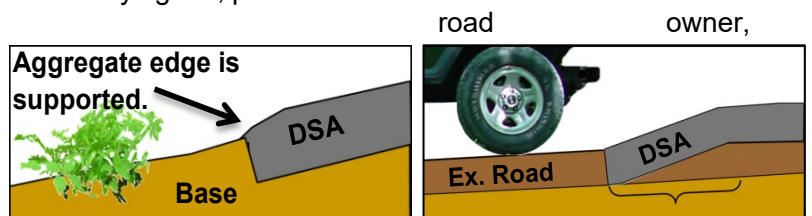
Reflect cross-slope in road base.
