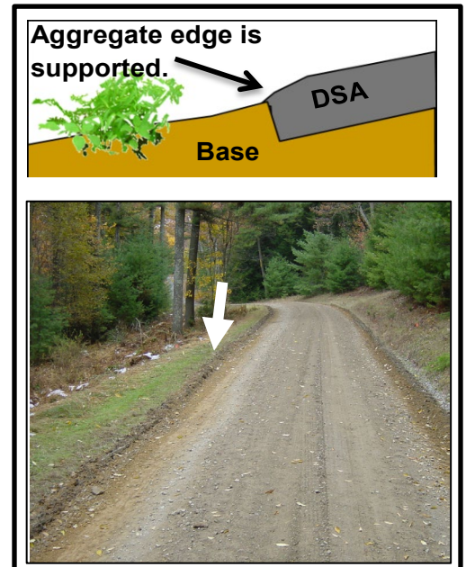
Figure 10. Key cut lengthwise along road prior to DSA placement
