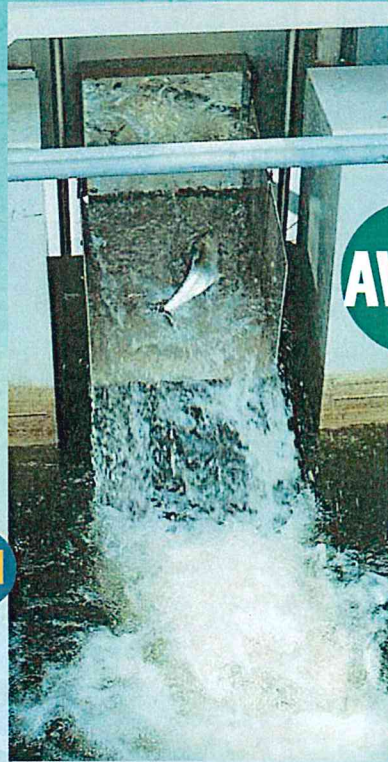
The fish lift at Safe Harbor Dam began operation in 1997. This fish lift, like Conowingo Dam's lift, passes migrating fish directly into the pool above the dam.
